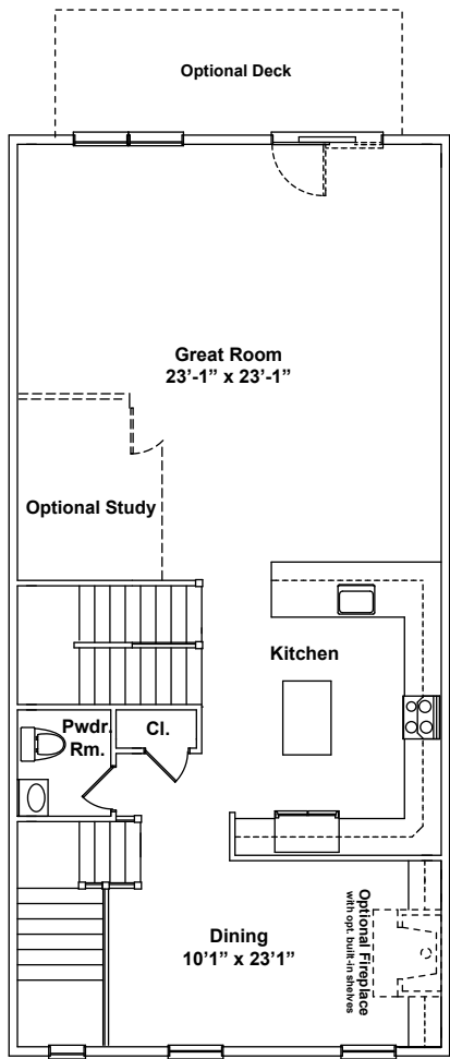
First Floor Centered Kitchen Elevation A
