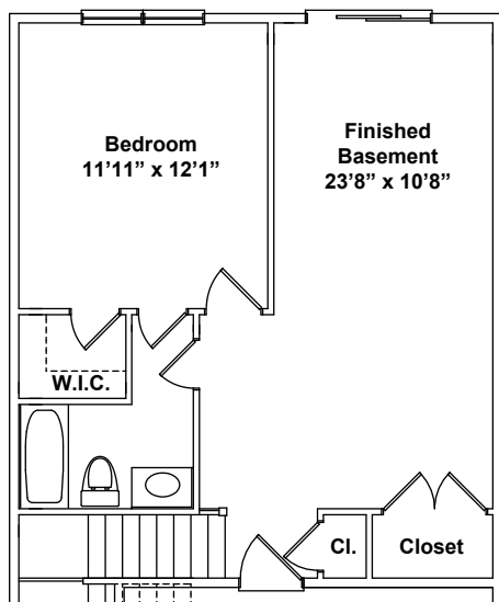
Partial Lower Level Plan with Bedroom and Bath Option
