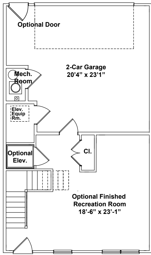
Lower Level Plan with Optional Finished Recreation Room
